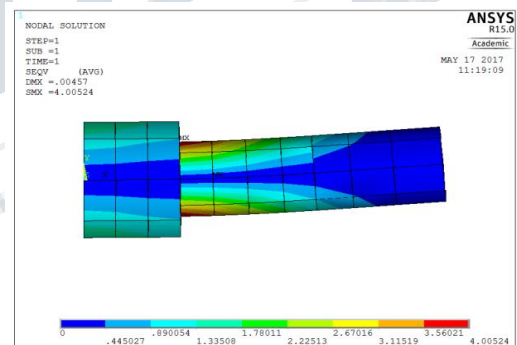
Fig.17 stress analysis of wheel shaft S1
