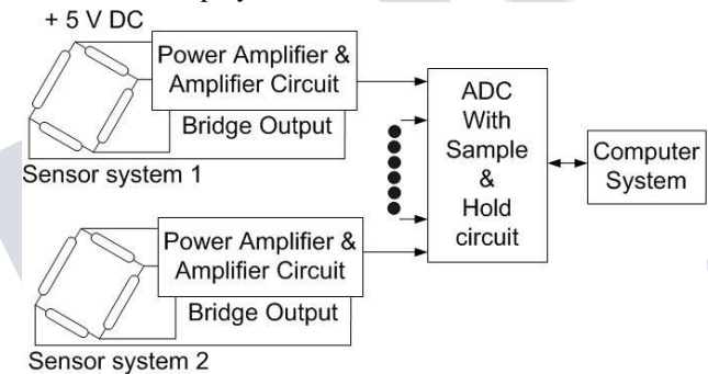
Fig. 2 Interface details of the sensing system
