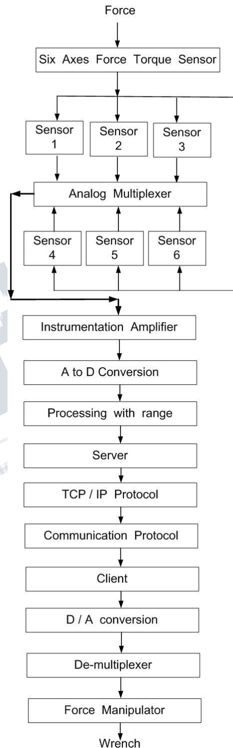
Fig. 4 Flow chart of the implemented software
