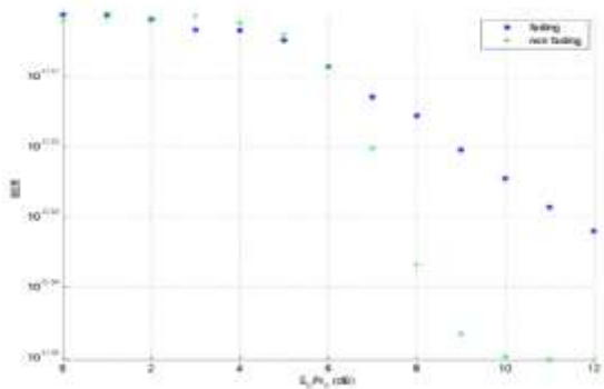
Fig:5: Effect on fading and Non Fading Channels
