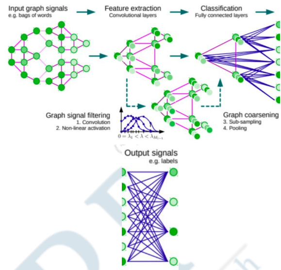
Figure 2: Use Filter Approach on the CNN
