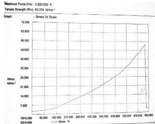
Fig. 17. Stress vs Strain graph for tensile test of Sample B2
