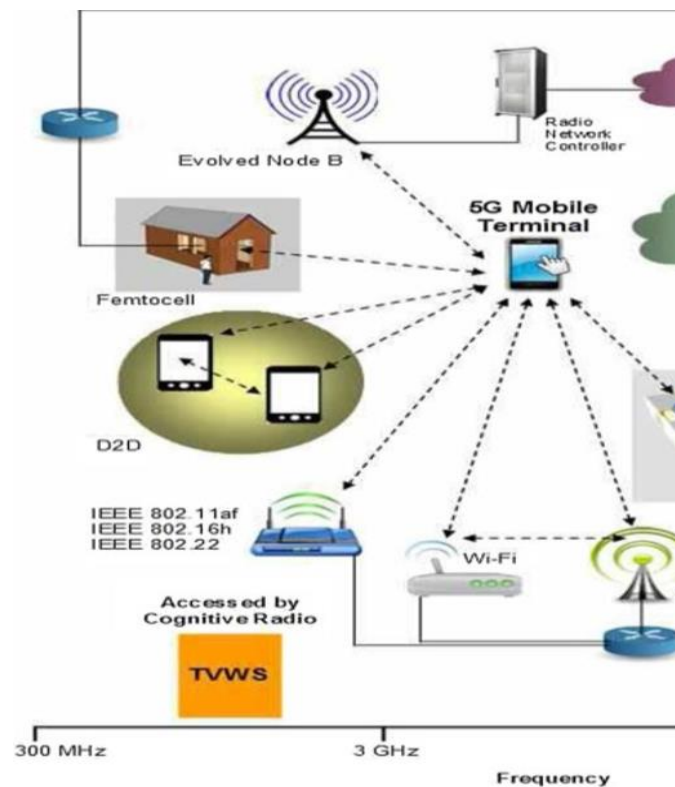
Fig.2: Traffic offloading approaches for fifth generation networks
