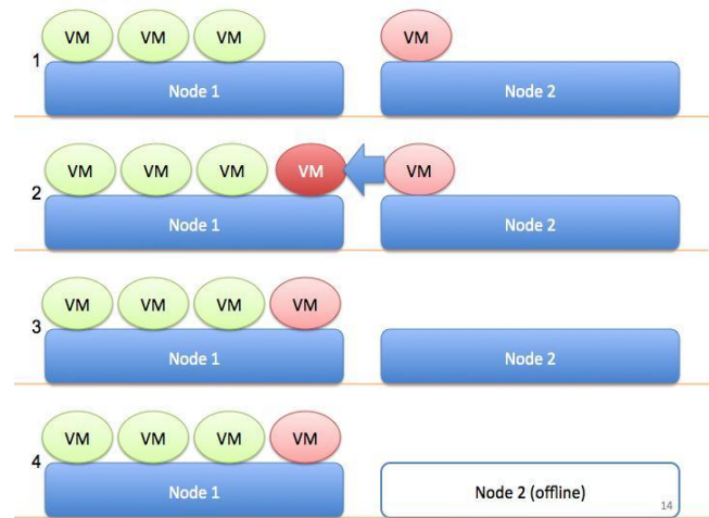
Fig. 6. Virtual Machine management dynamic shutdown technique
