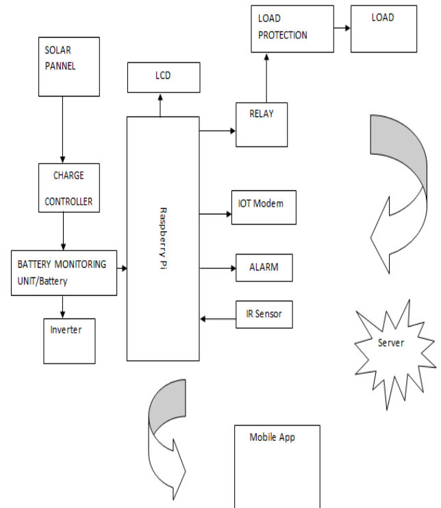
Fig 2. Block diagram of IoT based smart inverter using Raspberry pi
