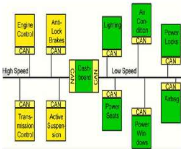
Fig 2. Block Diagram Of Proposed System (With CAN)
