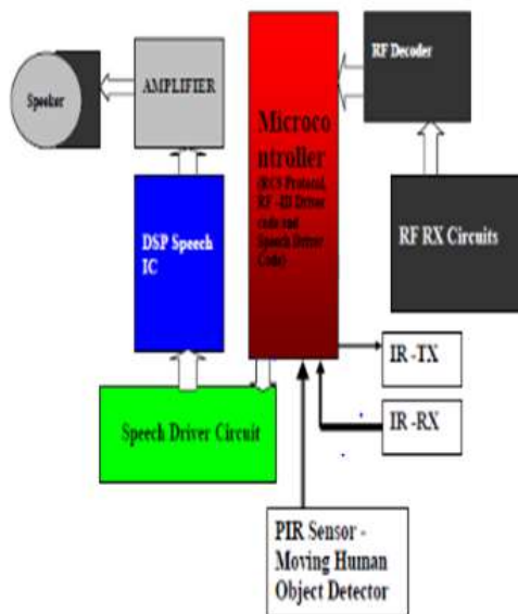
Fig.4: Block diagram
