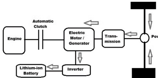
Figure.2: Regenerative Braking System for Automobile
