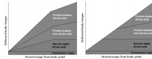
Figure.3: Parallel and Serial Regenerative Braking Control Respectively
