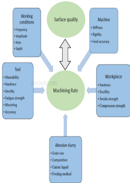
Figure 2: Static & dynamic machining
