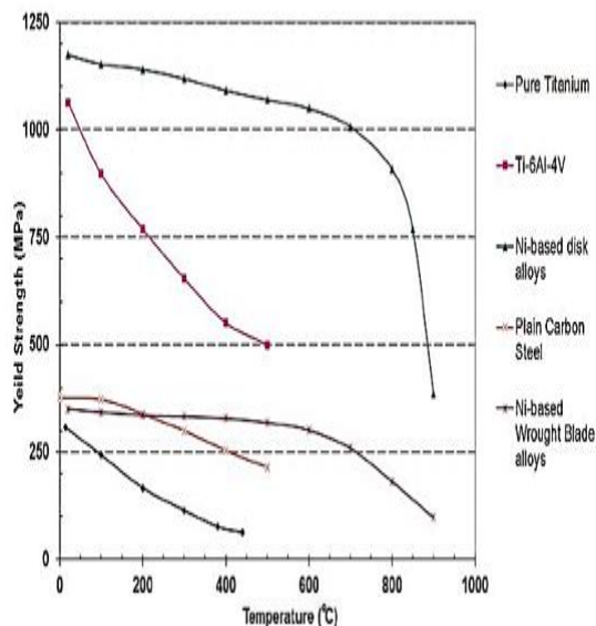
Figure 4: Yield strength Vs Temperature during machining process
