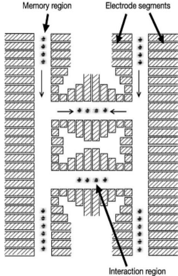
Figure 4: Quantum Charged Coupled Device (QCCD)
