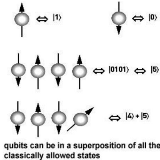
Figure 3: Qubits
