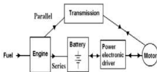
Figure 1: The Series or Parallel Path of an HEV Nevertheless, emissions from HEV remain. Introducing HEV plug-in solves some of the problem. It accepts electrical power from the mains to battery
