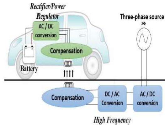
Figure 3: Diagram of Wireless charging system of electric vehicles
