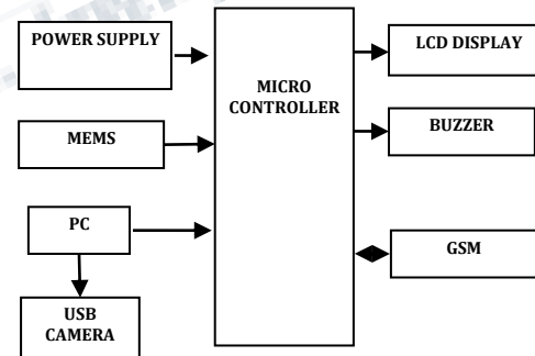
Fig 1: Block diagram
