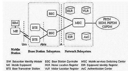
Fig 2:GSM architecture
