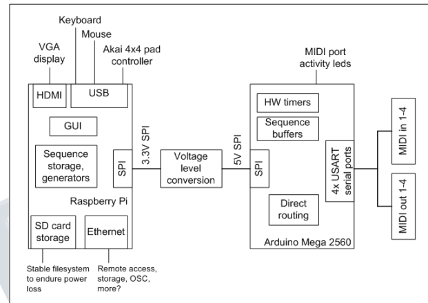
Project architecture
